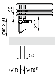
Detail: Connection fitting with long cover and integrated electric heating element WIVAR II.
