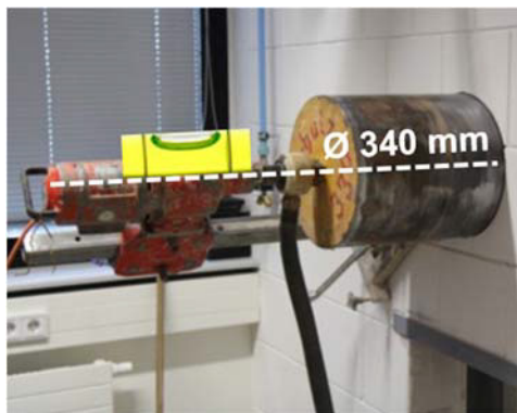
Fig. 2 Drilling the core hole
