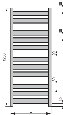
Front view PQ6(C)-120
