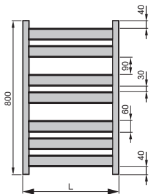
Front view PQ6(C)-080
