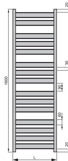
Front view PQ6(C)-160
